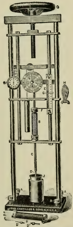
FIG. 165.—Consistometer.
